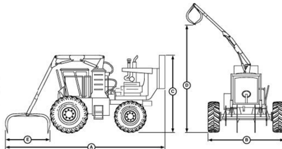
GAME 4700LX Loader Dimensions
